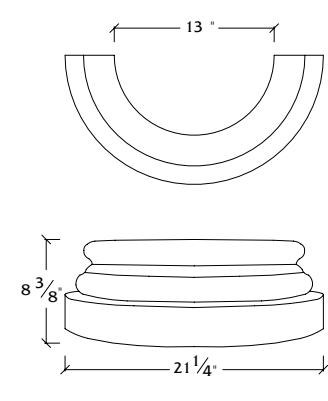
C-B-8 Base
