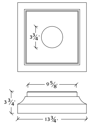
SC-B Base
