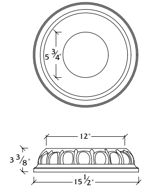
C-4 Collar
