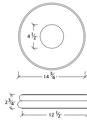
C-3 Collar
