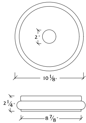
C-1 Collar
