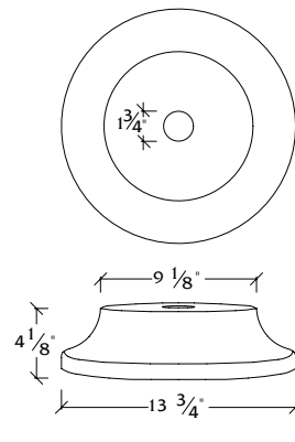
RC-B Base
