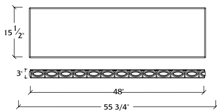
B-S-48* B-S-55* Bench Seat
