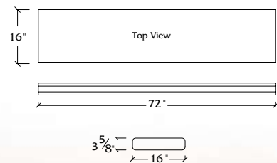
M-16-6 Bench Seat
