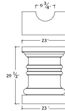
RC-10-24 Table Bottom
