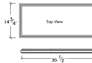
B-S-35 Bench Seat
