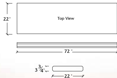
M-20-6 Bench Seat
