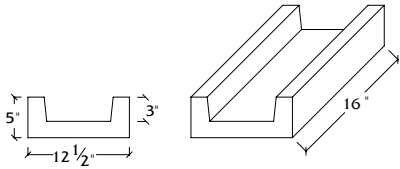
SC-1 Scupper
