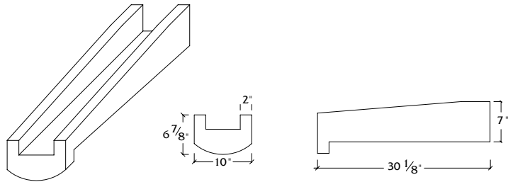
SC-5 Scupper
