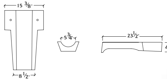
SC-6 Scupper
