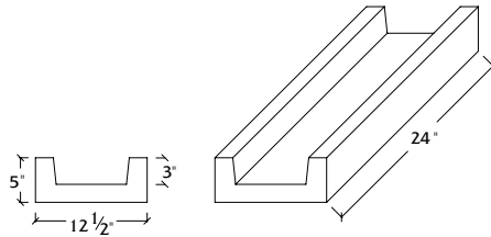
SC-2 Scupper
