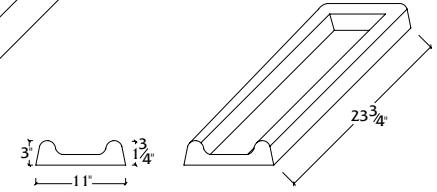
SB-D Splash Block
