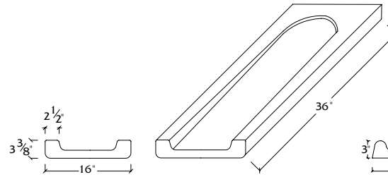
SB-C Splash Block
