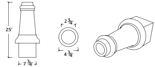
SC - 4 Cannon Scupper
