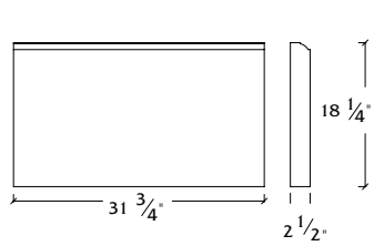
W-18-32 Wainscot
