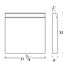
W-32-32 Wainscot
