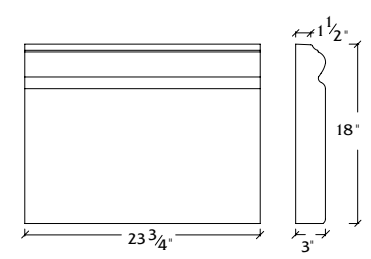
W-18-24 Wainscot
