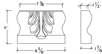
Leaf Plinth
