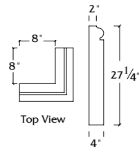
W-27-32C Wainscot
