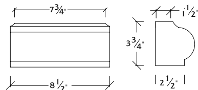
P-8B Plinth
