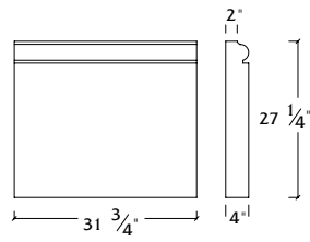
W-27-32 Wainscot
