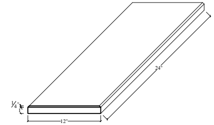
CHAMFERED PAVER
