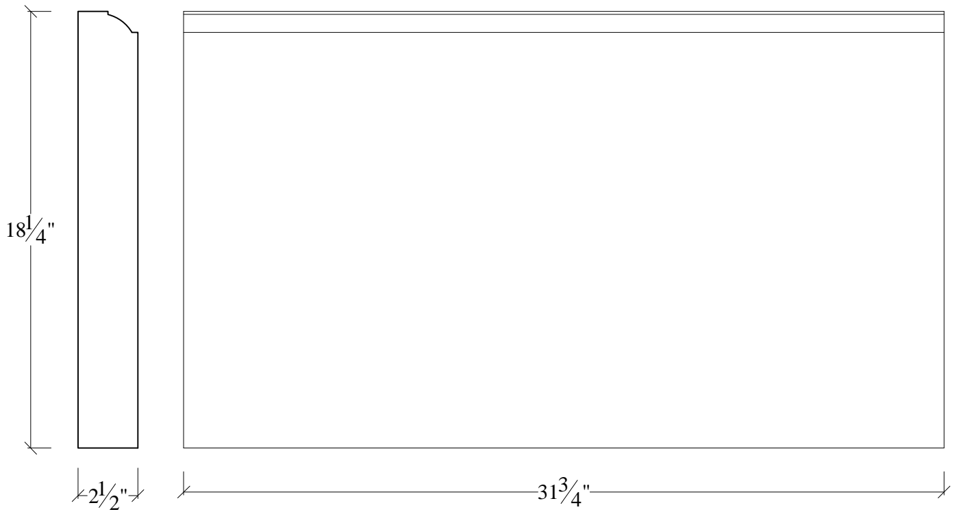
W-18-32 ( WAINSCOTT & PLINTHS)
