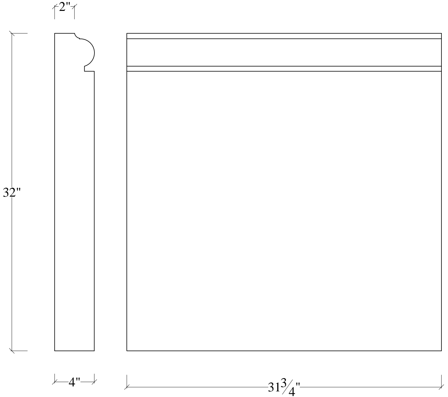
W-32-32 (WAINSCOTT & PLINTHS)
