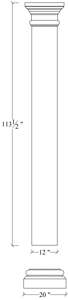
PROFILE
