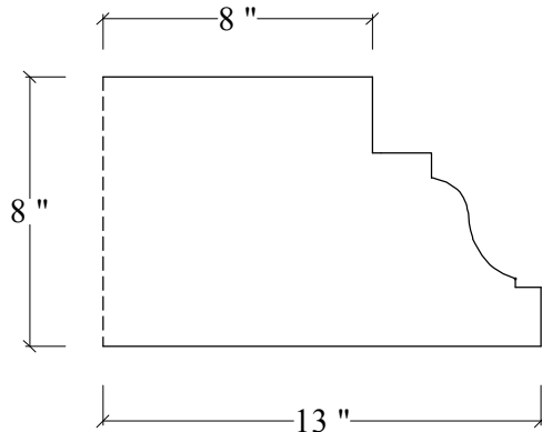
PROFILE
