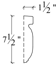
PROFILE
