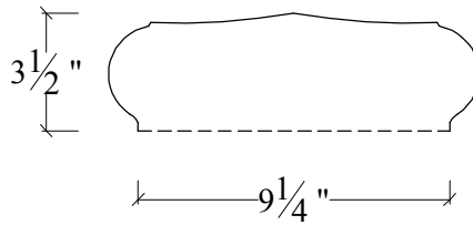
PROFILE
