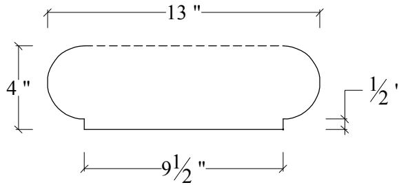
PROFILE
